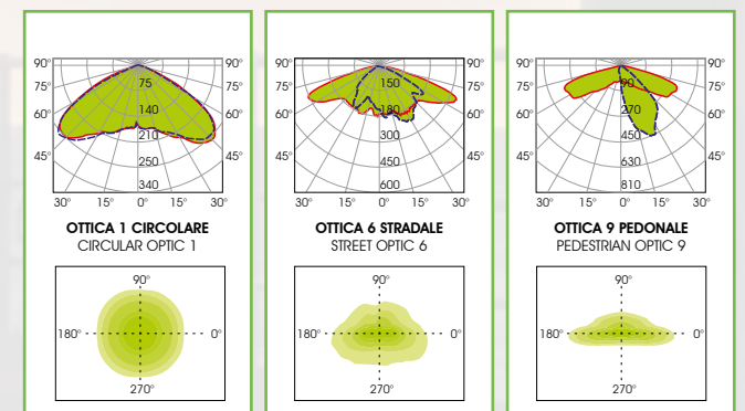
CURVE FOTOMETRICHE - PHOTOMETRIC CURVES
