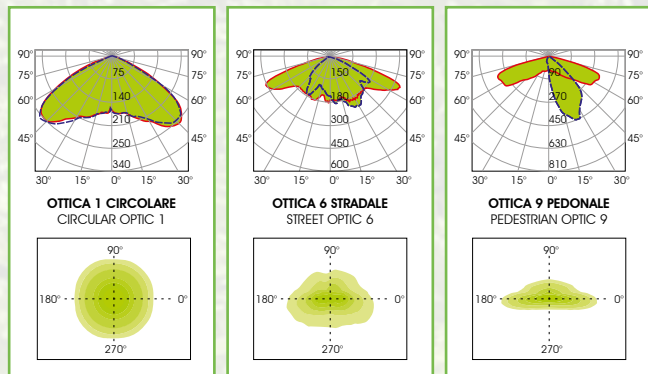
CURVE FOTOMETRICHE - PHOTOMETRIC CURVES
